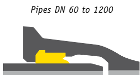
Pipes DN 60 to 1200
