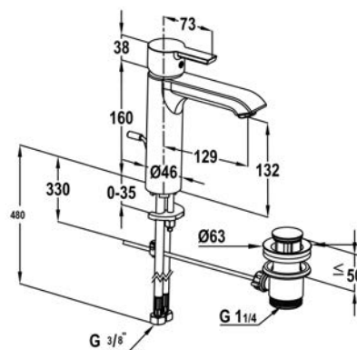
Dimensional drawing
